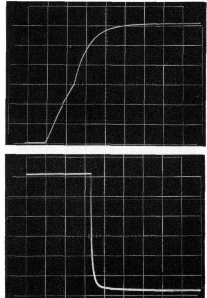
Fig. 8. Oscillograms of turn-on and turn-off characteristics of Model 722AR power supply. Both supplies have been designed to be free from spurious transients for protection to semiconductor or other low-voltage devices. Vertical scale is 10 v/cm; sweep time is 0.2 sec/cm.
